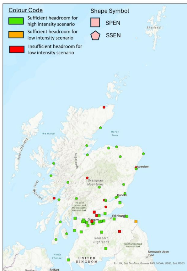
Figure 11. Substation capacity to support the core charger network and 2% of the HGV fleet reverting to BEV.
